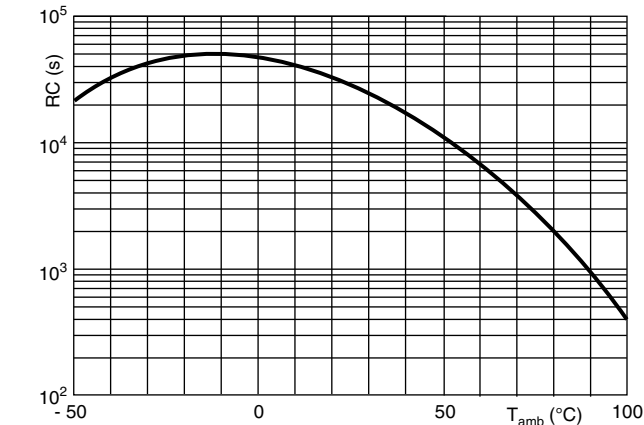
Insulation resistance as a function of ambient temperature (typical curve)
